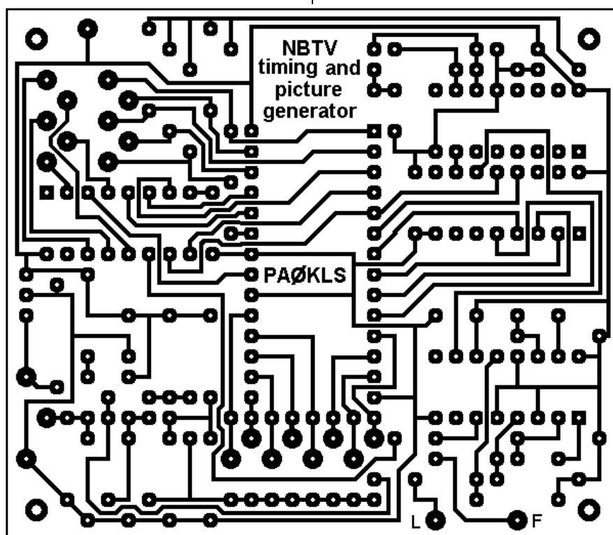
A printed circuit board
